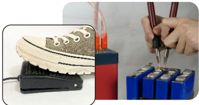
3. Hold the spot welding pen and press the welding needle tightly, step on the wire-controlled foot switch to trigger spot welding, and observe and check that the real-time welding current on the display should be within the range of 2.8~3.3KA (2800~3300A).
