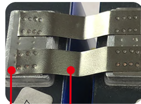
4. Check the spots' reliability. Finish spot welding.
